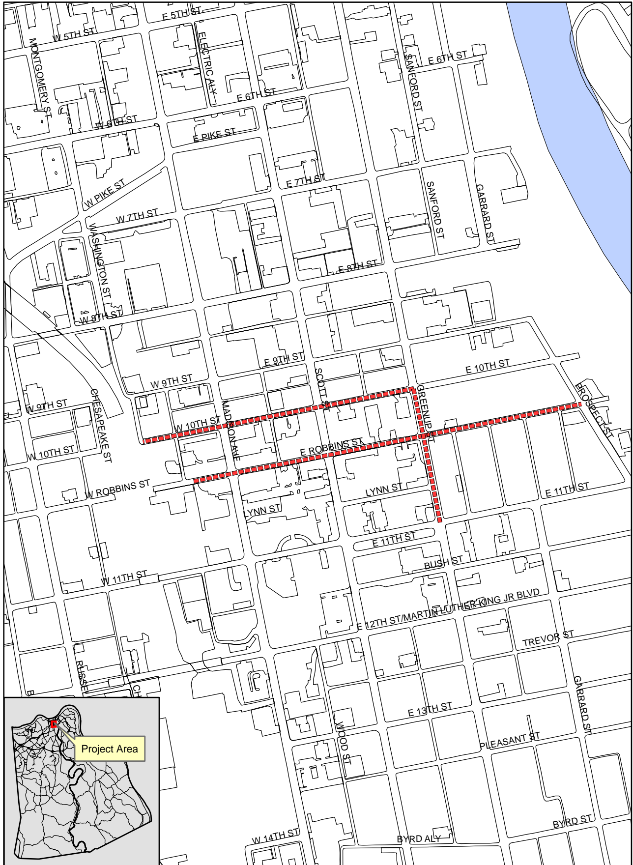
Robbins, Greenup, & 10th Street Water Main Replacement
