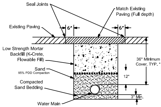
UNDER ASPHALT CONCRETE PAVEMENT
