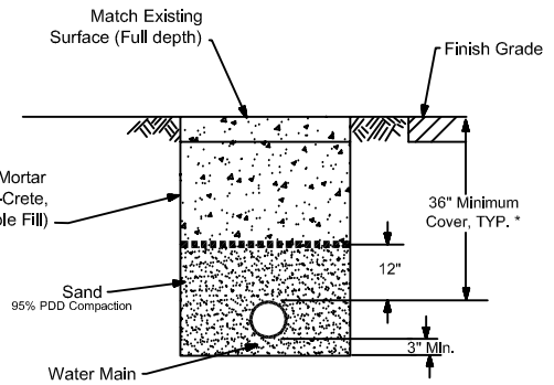
UNDER SHOULDER OF STATE MAINTAINED STREET
