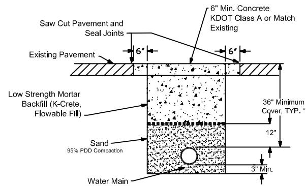
UNDER STATE MAINTAINED STREET
