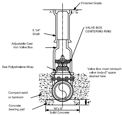
Detail Valve Box Installation
